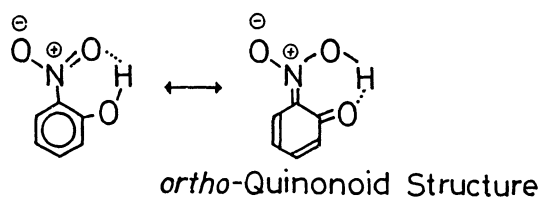
Fig. 1. Quinonoid structure of o -hydroxynitrobenzene.
